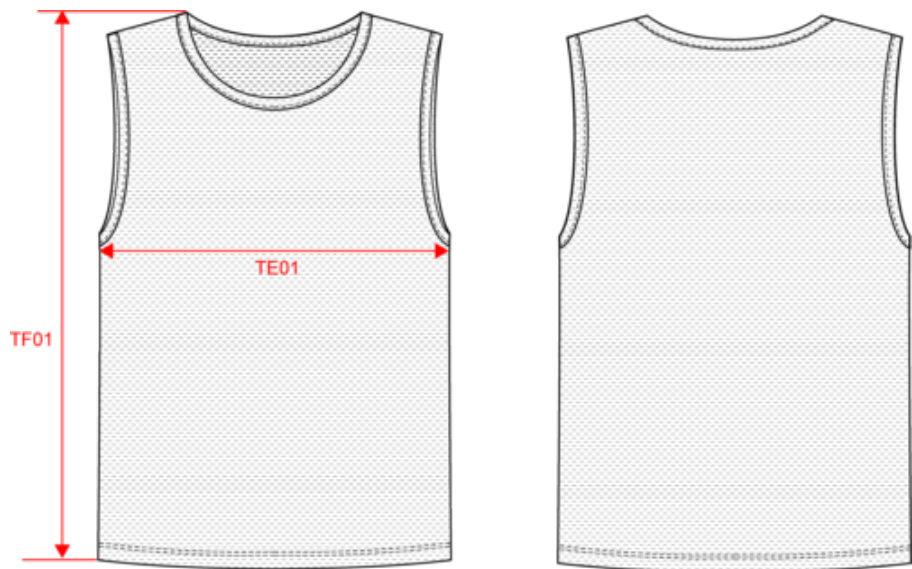
Dimensions (cm)
